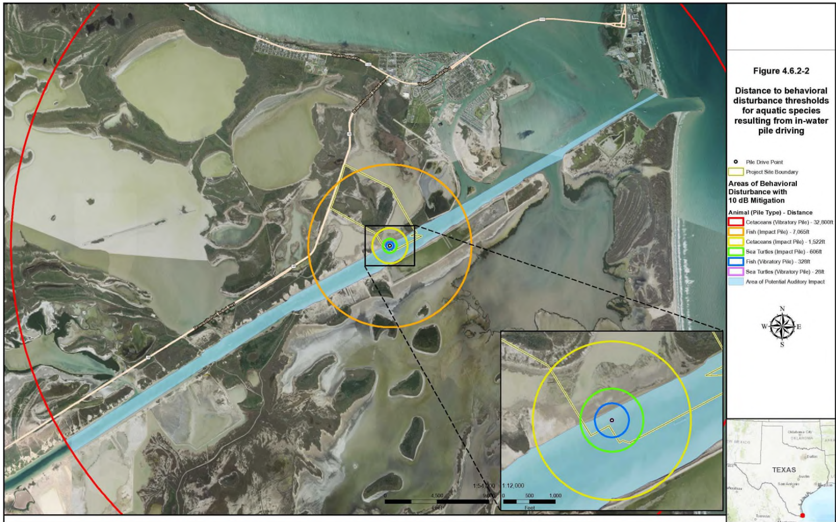
FIGURE 4.6.2-2 Distance to behavioral disturbance thresholds for aquatic species resulting from in-water pile driving.
