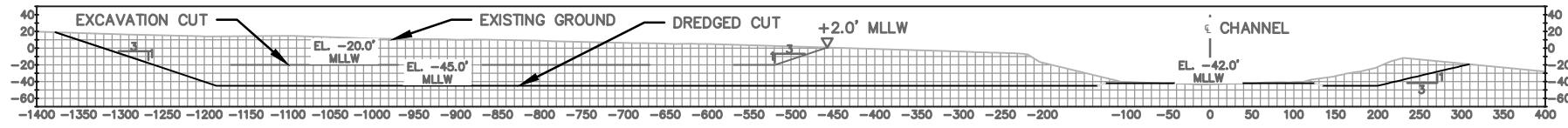
A1 SECTION AT WEST END MOORING DOLPHINS W-0006
