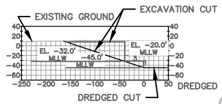
E1 SECTION AT MATERIAL OFFLOADING FACILITY (MOF) W-0006
