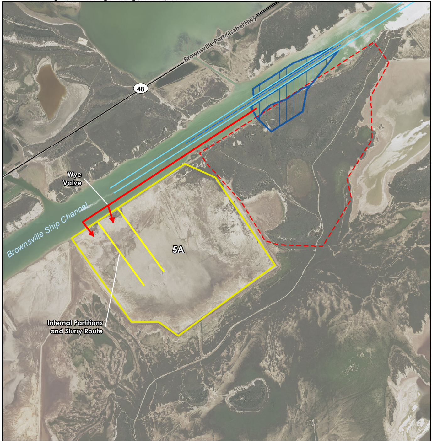
Figure 6 Hydraulic Dredge Pipeline Route Annova LNG Brownsville Project Cameron County, Texas
