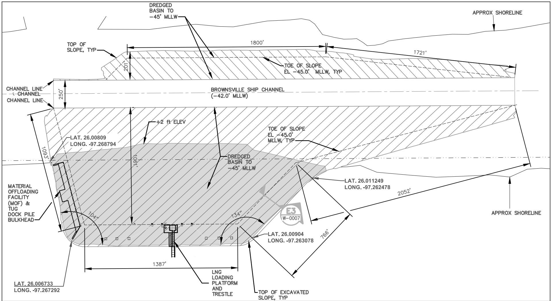
FIGURE 2 REV 1 DREDGING FOOTPRINT, PLAN VIEW ANNOVA LNG BROWNSVILLE PROJECT CAMERON COUNTY, TEXAS
