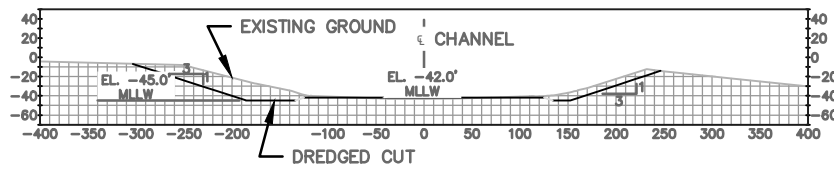
E6 SECTION AT HEAD OF BASIN W-0006
