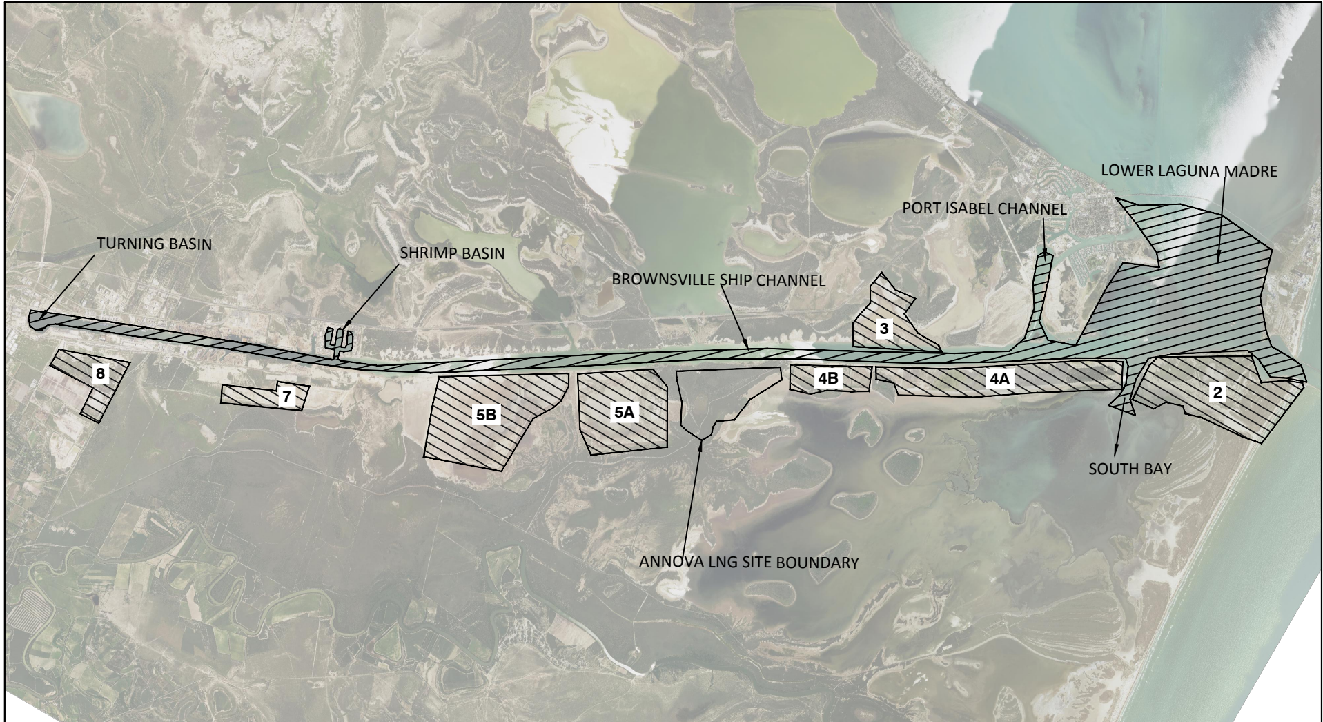
FIGURE 4 BROWNSVILLE NAVIGATION DISTRICT DREDGED MATERIAL PLACEMENT AREAS ANNOVA LNG BROWNSVILLE PROJECT
