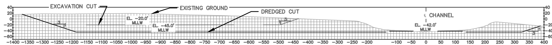
D1 SECTION AT EAST END MOORING DOLPHINS W-0006
